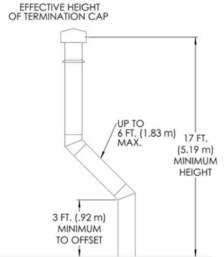
Figure 23 - Typical Residential Installations
