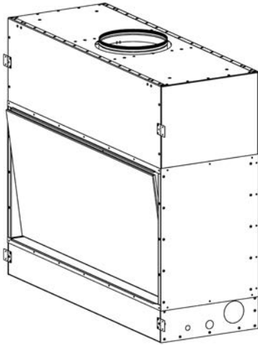
Figure 36 - Rear Panel Installation
