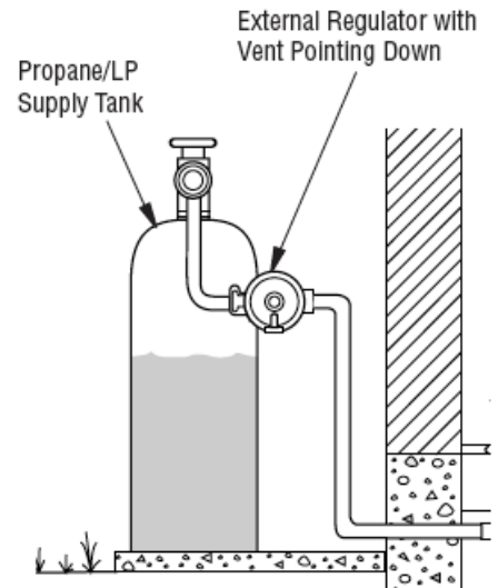
Figure 25 - External Regulator with Vent Pointing Down (Propane/LP Only)
