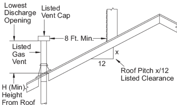
Figure 22 - Typical Terminations
