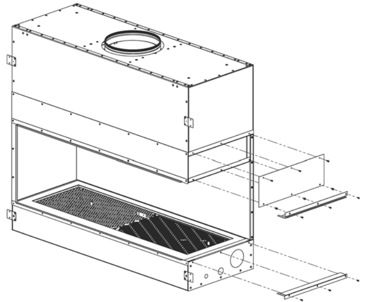
Figure 42 - Left Reduction Kit
