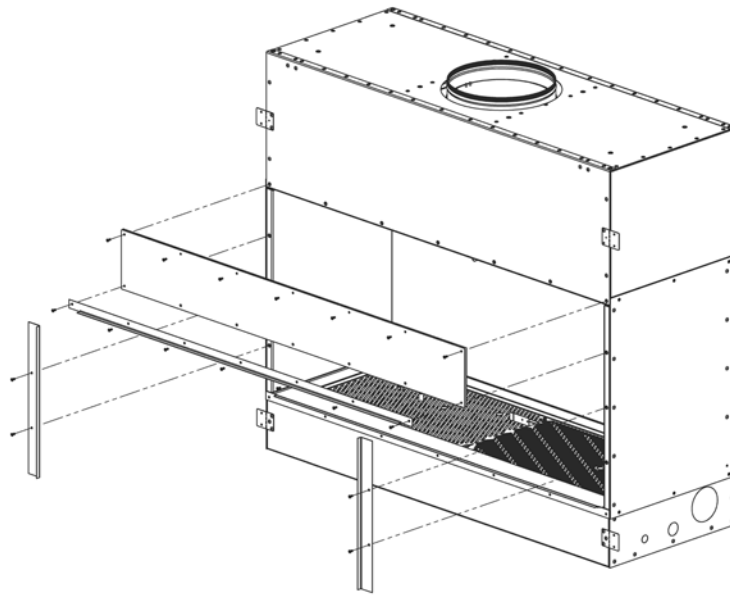
Figure 40 - Front Reduction Kit
