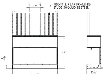
FRONT ELEVATION
